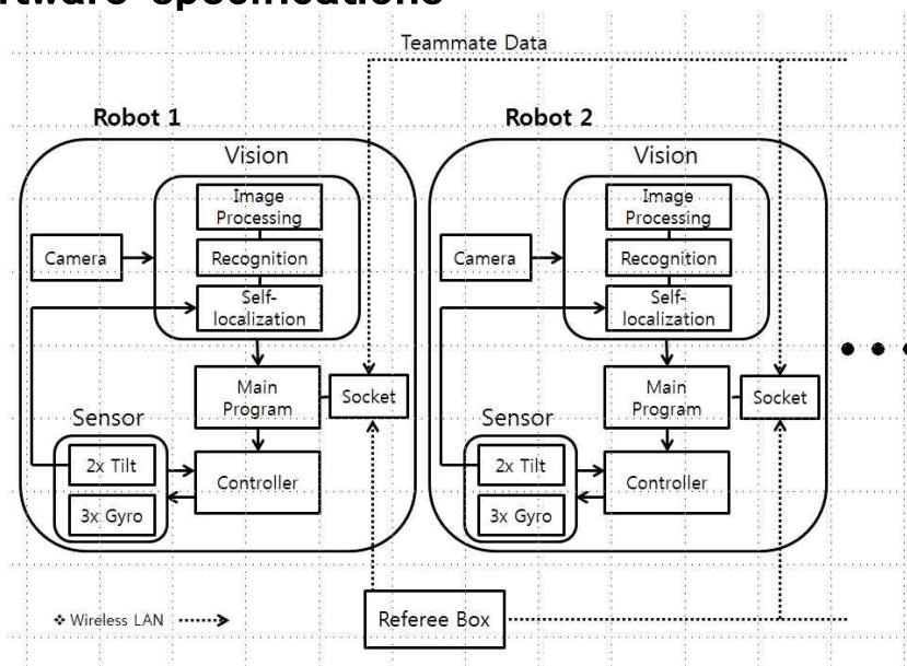
< Figure 4.1 SoftWare >
