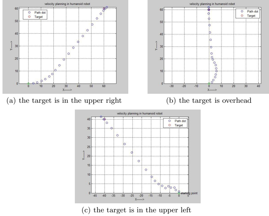
Fig. 4. Velocity planning in humanoid robot
