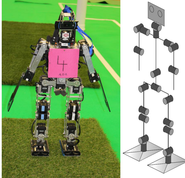
Fig. 1: Current model (left) and its kinematics (right)
