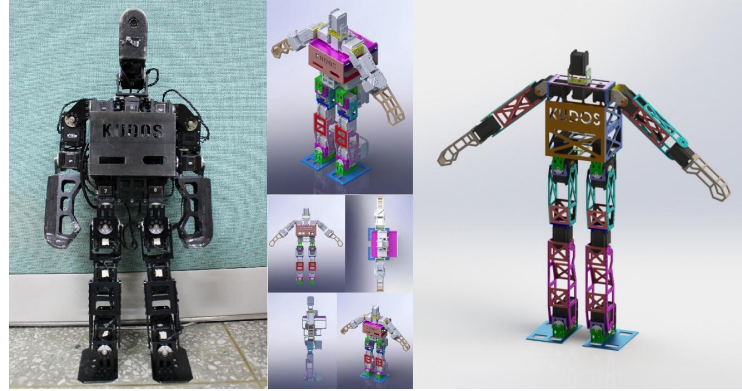
Fig. 2. 3D-printed KUbota2 and Design of KUbota2 and KUbota-teen
