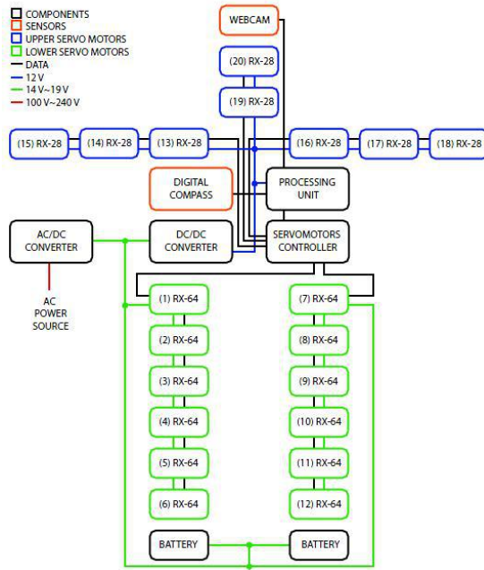
(a) Connection block diagram
