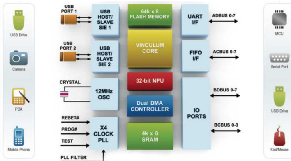
Figure 3 VNCL1-1A application and performance block diagram
