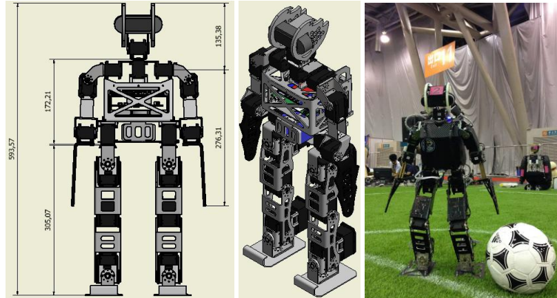
Figure 2. The layout of Mechanical structure and the dimensions of EROS robot.
