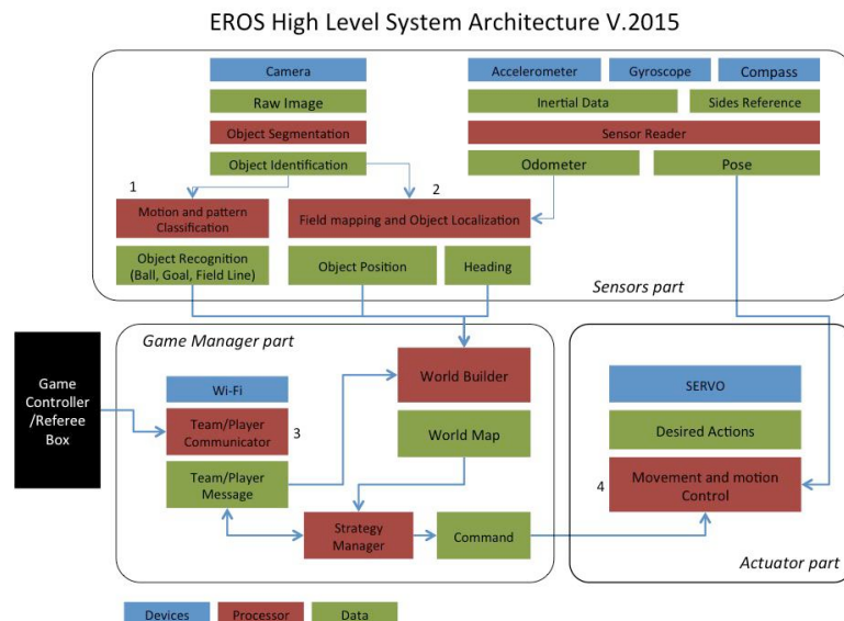
Figure 3. The latest system architecture customized 1, 2 in the image processing and system odometer. 3 in the game managers part and 4 in the actuator part.
