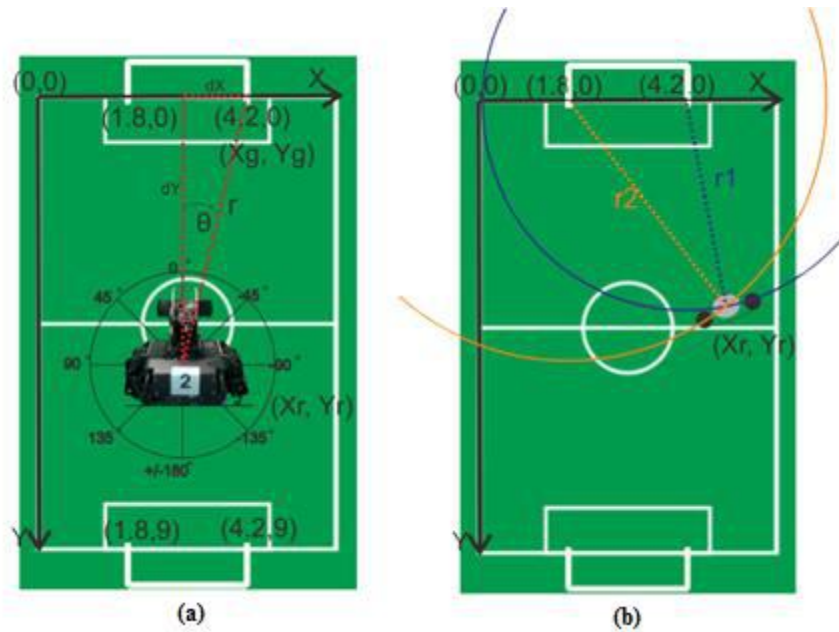
Fig. 4. Robot Orientation using Trigonometry (a) and Triangulation (b)
