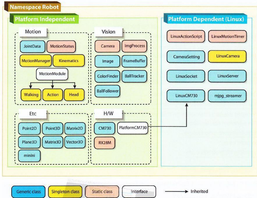
Fig. 1. Darwin-OP Framework Class Library Diagram
