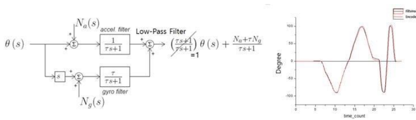
Fig. 6. Complementary Filter Block diagram and Graph
