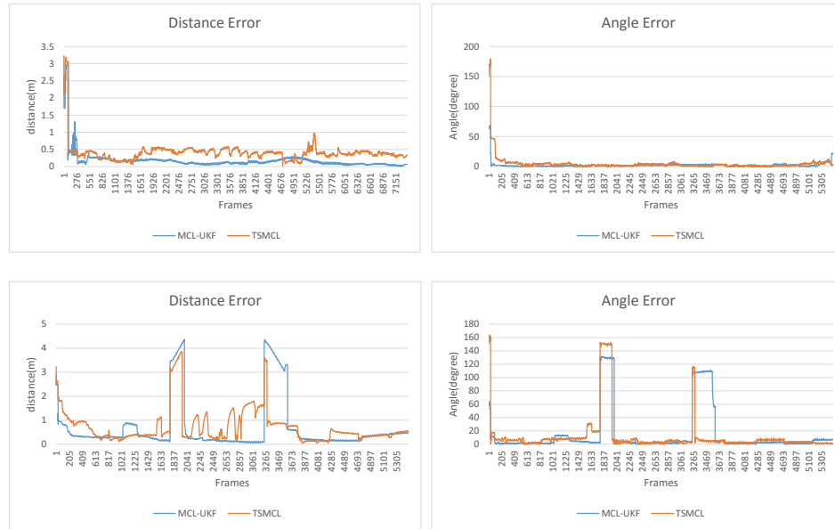
Fig. 2- Results of the accuracy and relocalization experiments. Top row shows the accuracy and bottom row shows the ability to recovering from kidnap.
