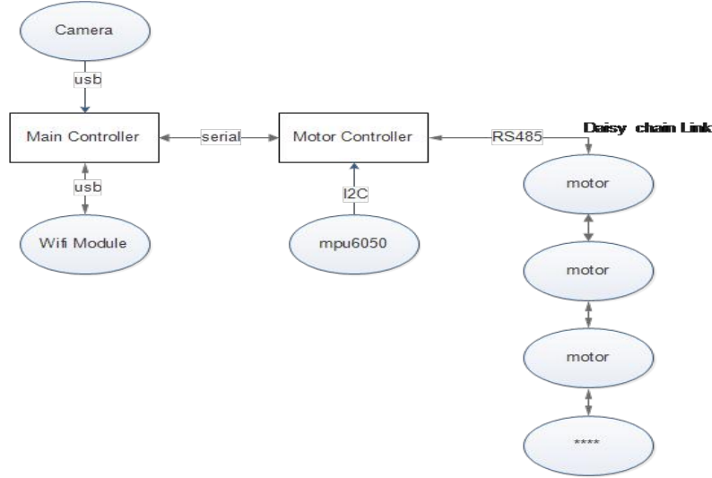
Figure 3: Electrical Architecture
