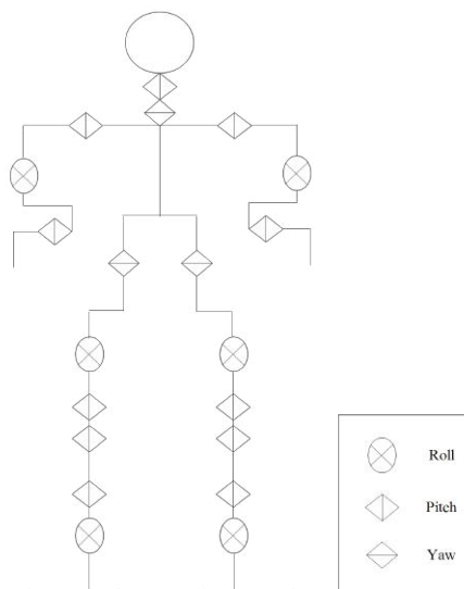
Figure 2: Actuator
