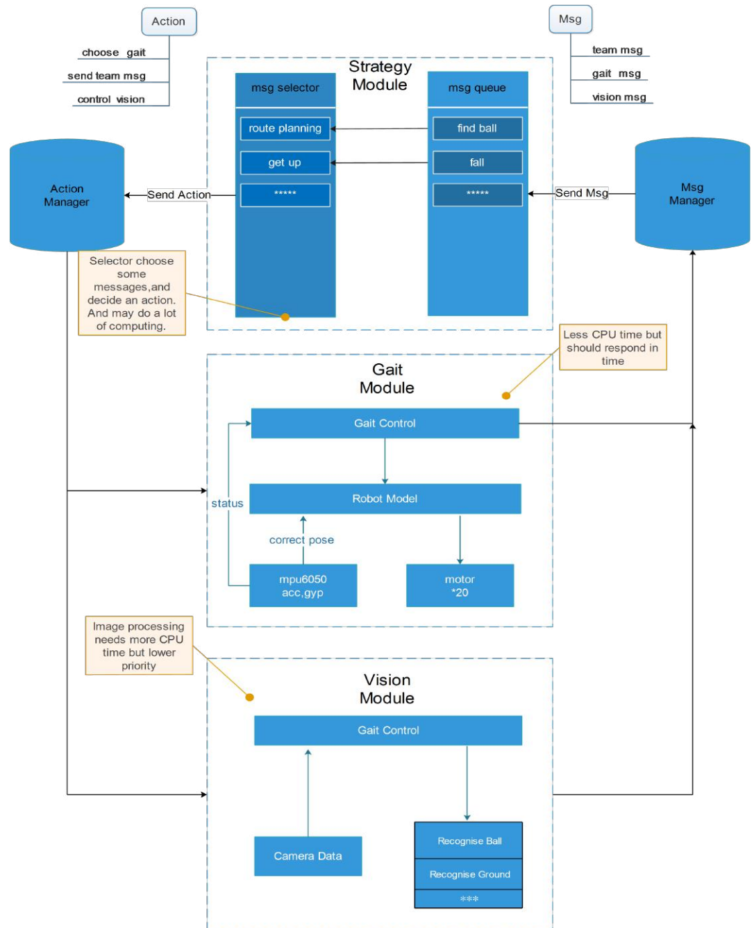
Figure 4: Software Architecture
