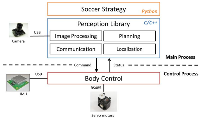
fig. 2. Overview of Software architecture
