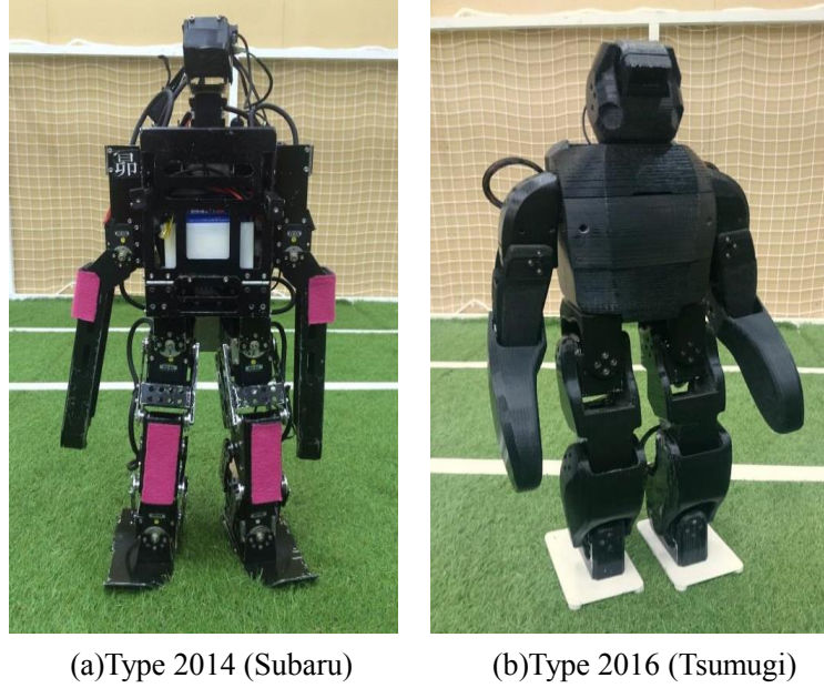
Fig.1. Developed robot.
