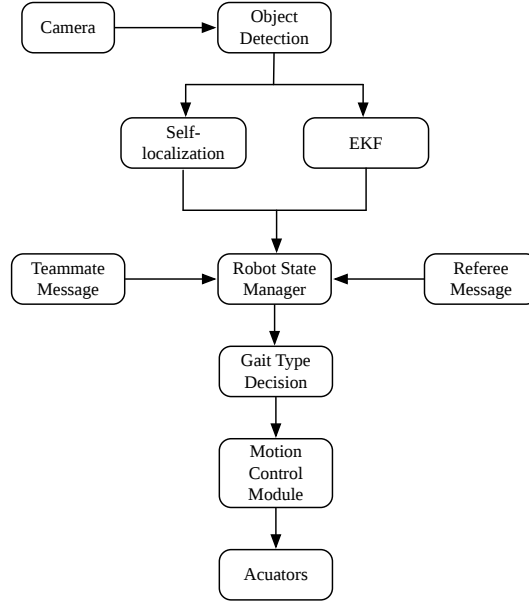
Fig. 3: Software Architecture
