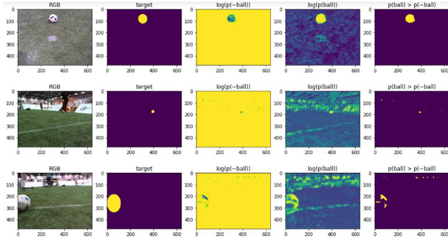
Fig. 3: Segmentation results of a FCN with less than 2000 parameters, achieving 99.4% accuracy on ball segmentation: ignoring penalty mark, far ball on edge of field, moving ball.
