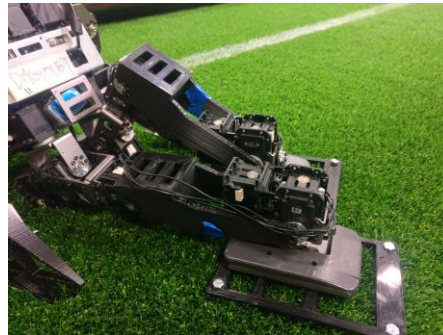
(b) 3D printed legs.
