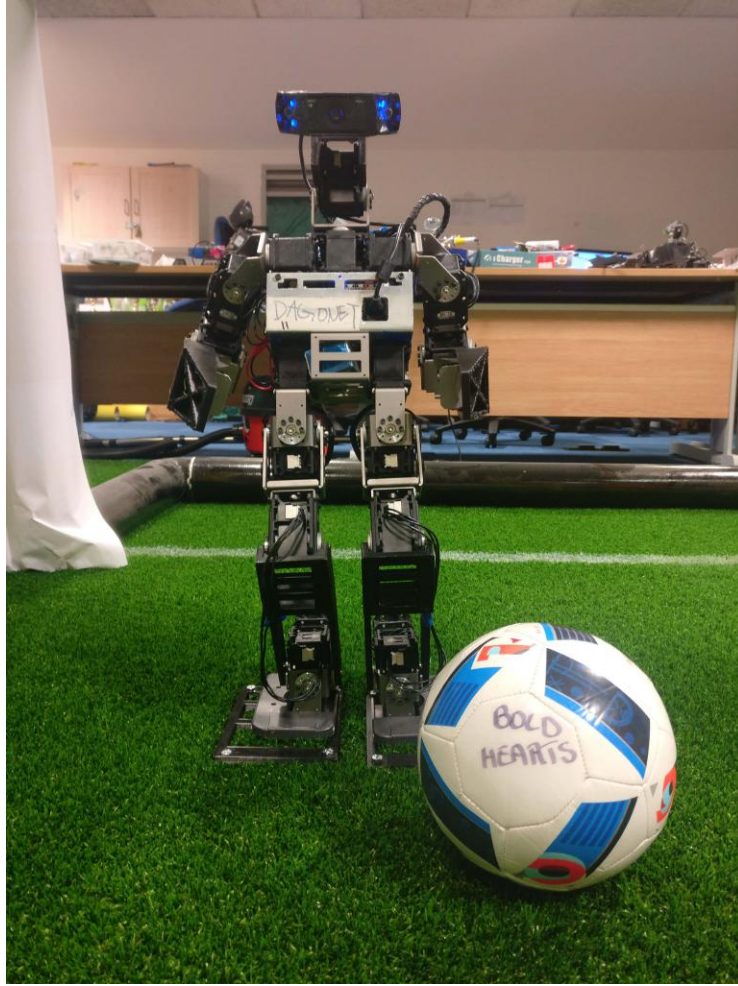
Fig. 2: An example of the new platform “Boldheart 2”: It has been assembled with a new computational unit (Odroid-XU4), a new camera (Logitech HD Pro Webcam C910) and self-designed torso, feet, arms, legs and a head.
