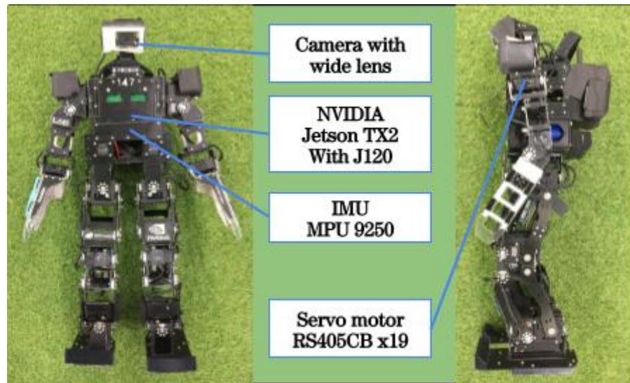
Fig. 2 Structure of the Accelite
