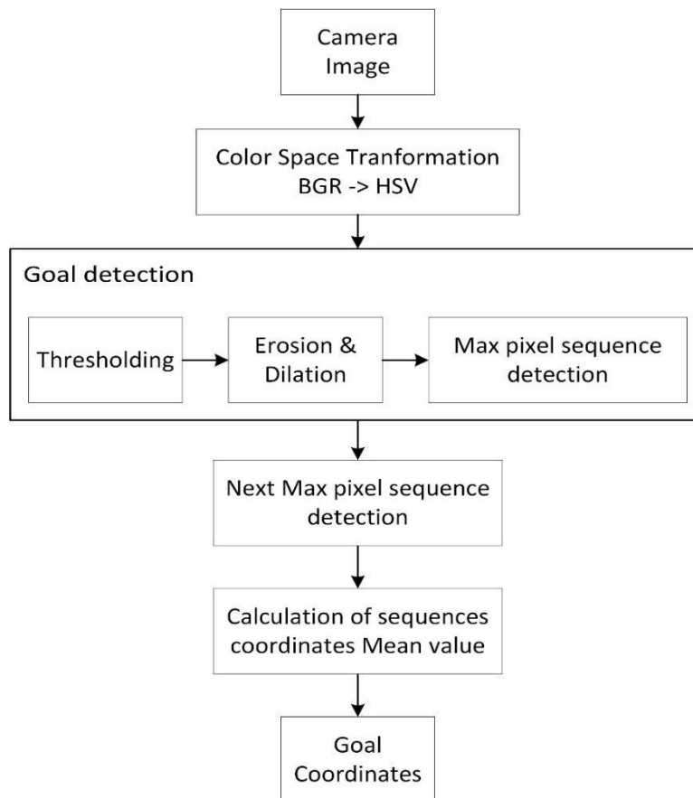
Fig. 3. Goal Recognition Algorithm
