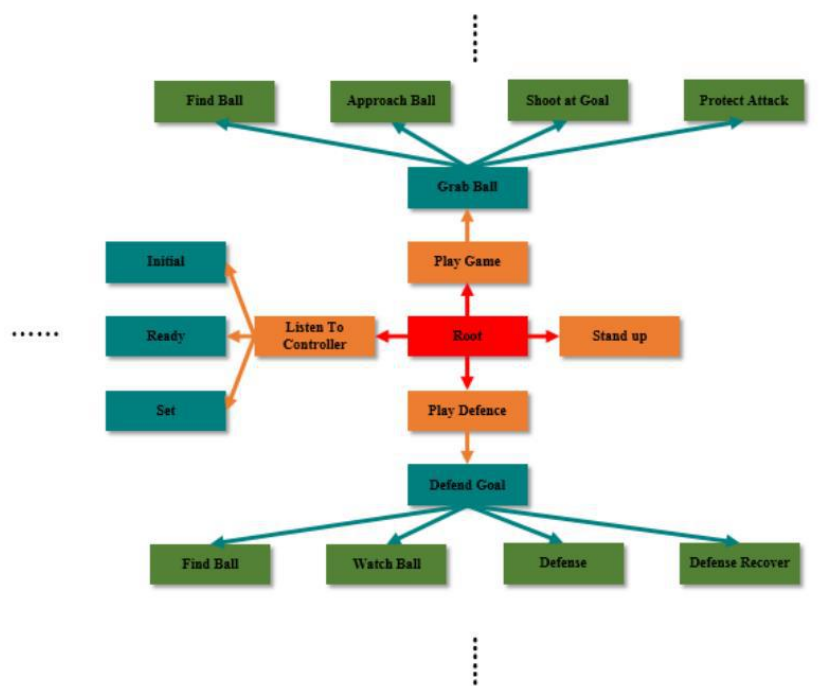
Fig. 7. A simplified option graph of robot behavior
