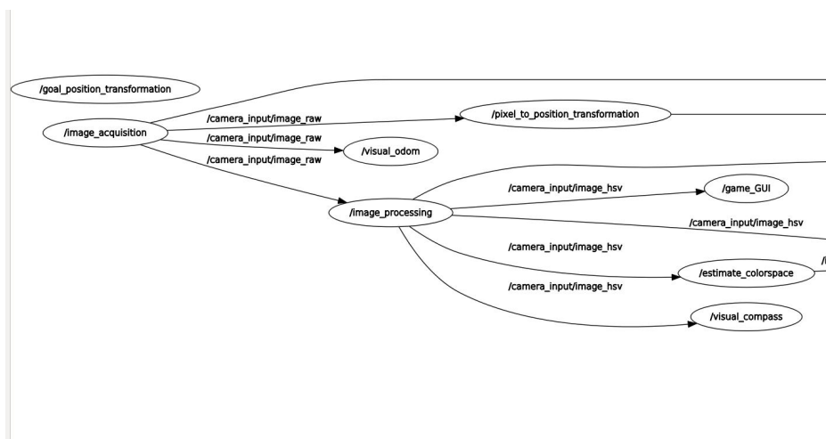
Fig. 5. ROS graph of computer vision inputs.
