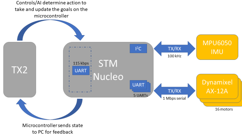
Fig. 4. Interfaces with NVIDIA Jetson TX2 and peripherals.
