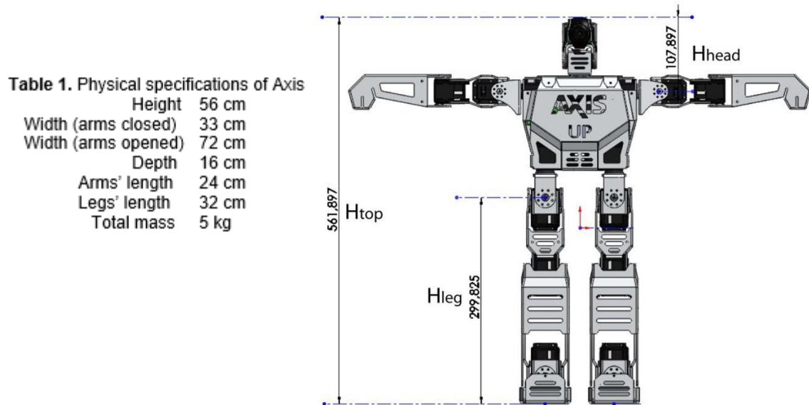
Fig. 5. Physical dimensions of VATIO-UP Humanoid Robots
