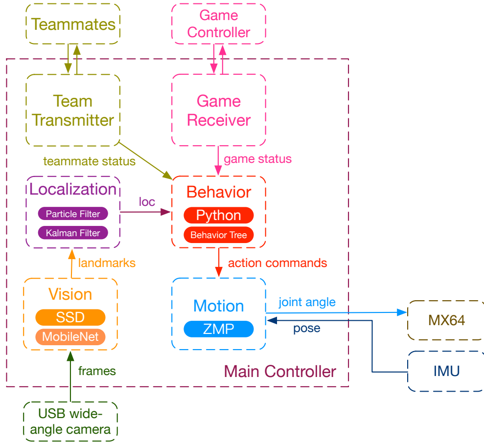
Fig. 4: Software Architecture
