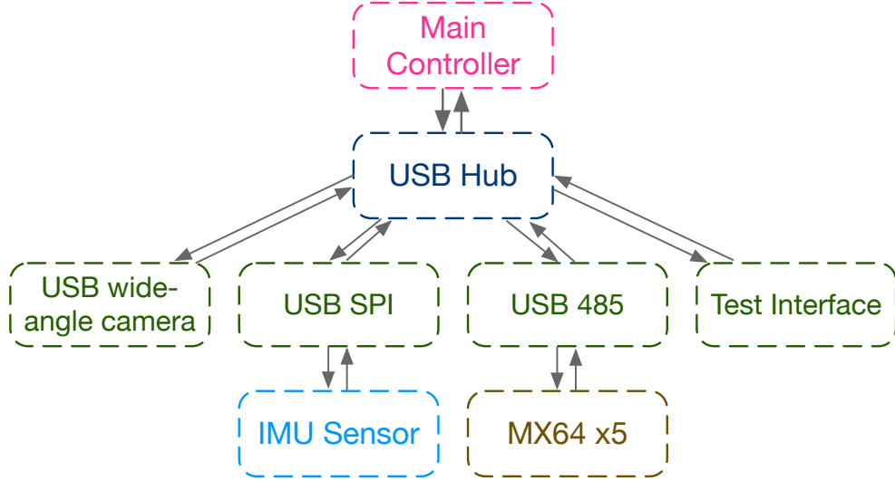
Fig. 3: Hardware Architecture
