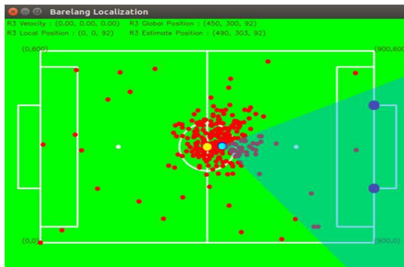
Fig. 9. Position predictions from particle filters.
