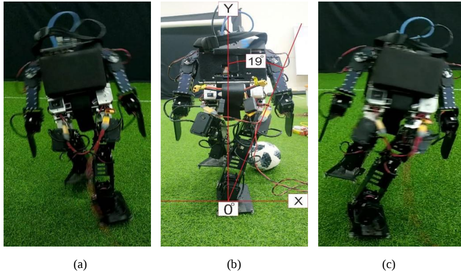
Fig. 10. Robot behavior when side kick (a) less than 18^\circ (b) 19^\circ \pm 1^\circ (c) greater than 21^\circ .
