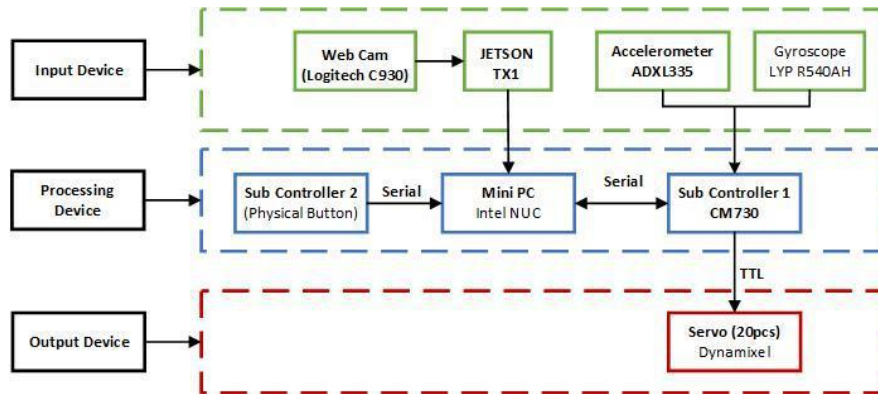
Fig. 1. Block diagram of hardware system.
