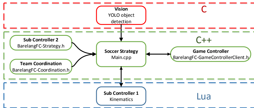
Fig. 2. Block diagram of software system.
