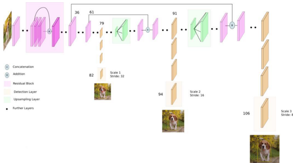
Fig. 5. YOLO v3 network architecture.
