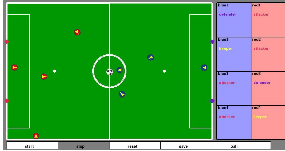
Fig. 5. Strategy Simulator.
