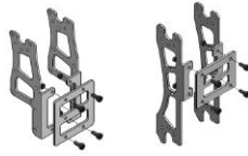
Fig. 3: A formed link of the robot using an aluminum angle
