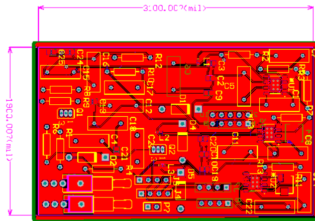
Fig.7. PCB sketch
