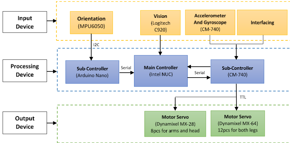
Fig. 1. Block diagram electronic system of Ichiro Robot
