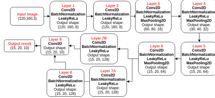
Fig. 6. Flow chart of the convolutional neural network we built. The image show also the shape of the output data for each layer. The names for each function used within layers are defined in Keras documentation [5].
