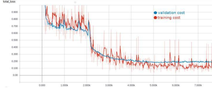
Fig. 5. Convergence of the model for regression of field boundary.
