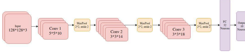
Fig. 4. Convolutional neural network for field boundary detection.
