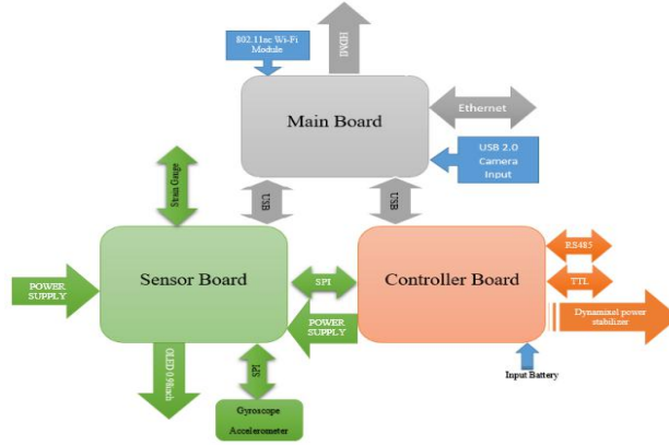
Fig. 2. System Overview
