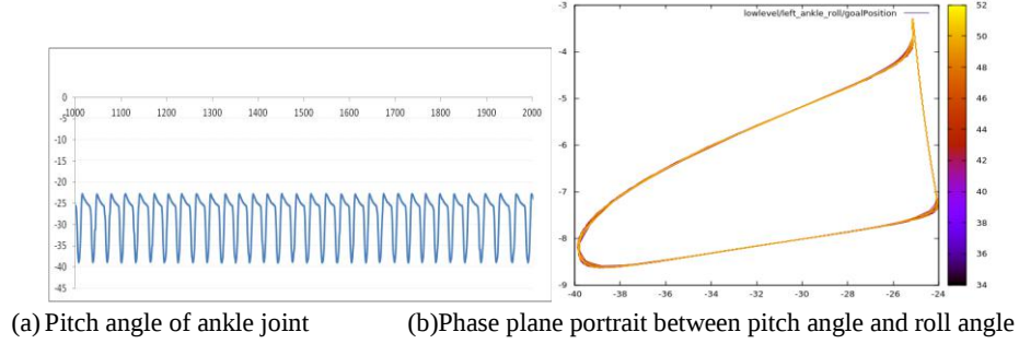
Fig. 2. Some output parameters of robot gait model.
