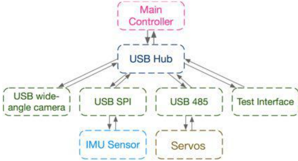
Fig. 3: Hardware Architecture
