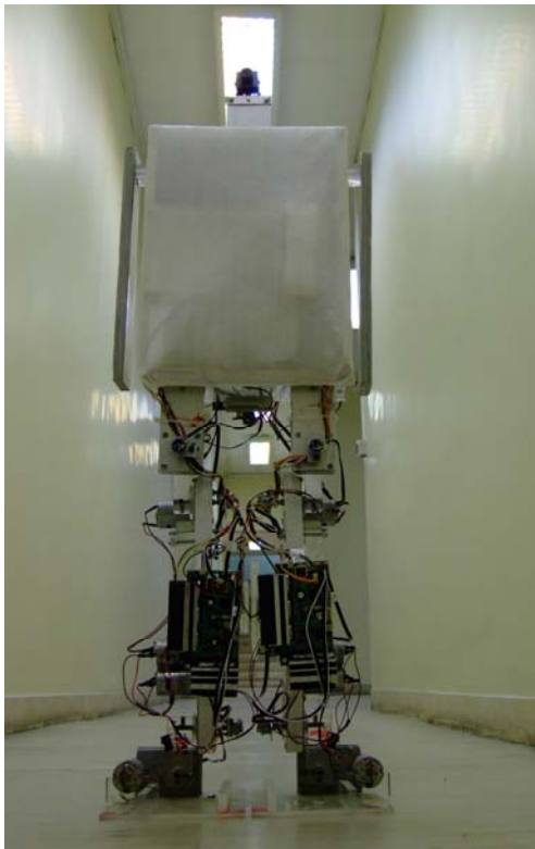
Fig.1. IranFanAvaran's 3rd Teen Size Robot, year 2008
