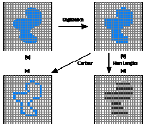
Fig.6. Algorithms to describing object contour
