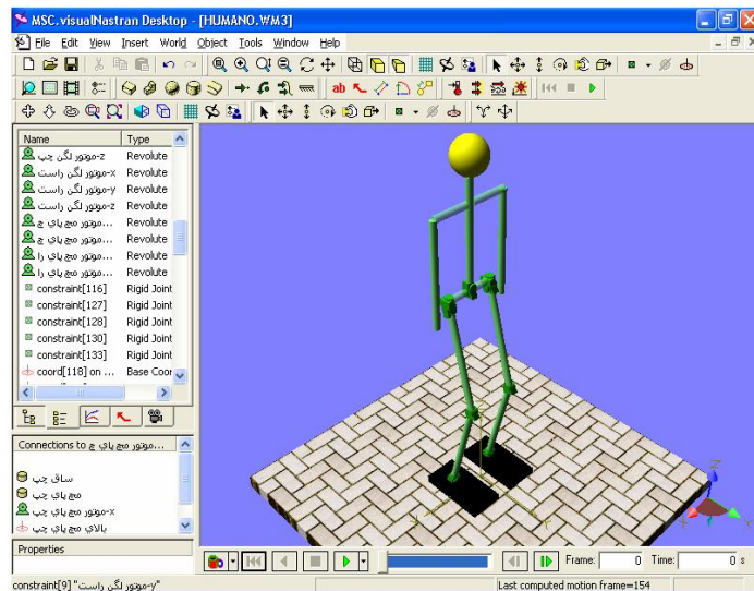
Fig.2. Modeling of the robot in Visual Nastran environment
