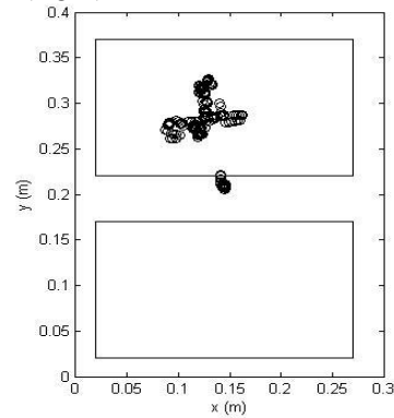
Fig. 7. ZMP distribution in kicking motion.
