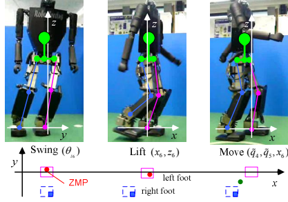
Fig. 2. The three action primitives defined in biped walking
