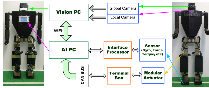
Fig. 1. Block diagram for RESr-III hardware control.
