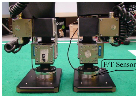
Fig. 6. Force/Torque sensors in the ankles.
