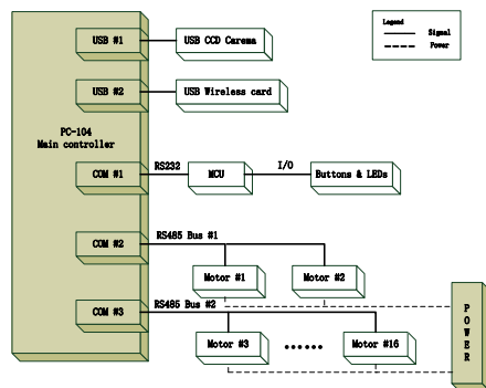
Fig. 2-3. The electrical system architecture of Stepper_Teen
