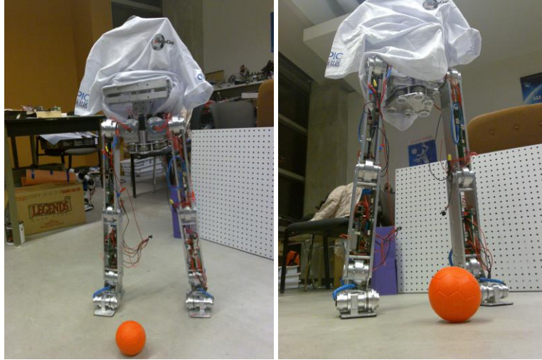
Fig. 1. ARCHIteen sized robot
