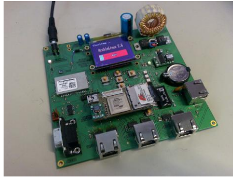
Fig. 5. ARCHIE: Spinal Processing Unit
