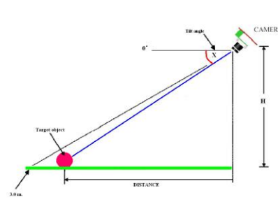
Fig. 7. Determination of the distance from the robot to the target object (Side View)
