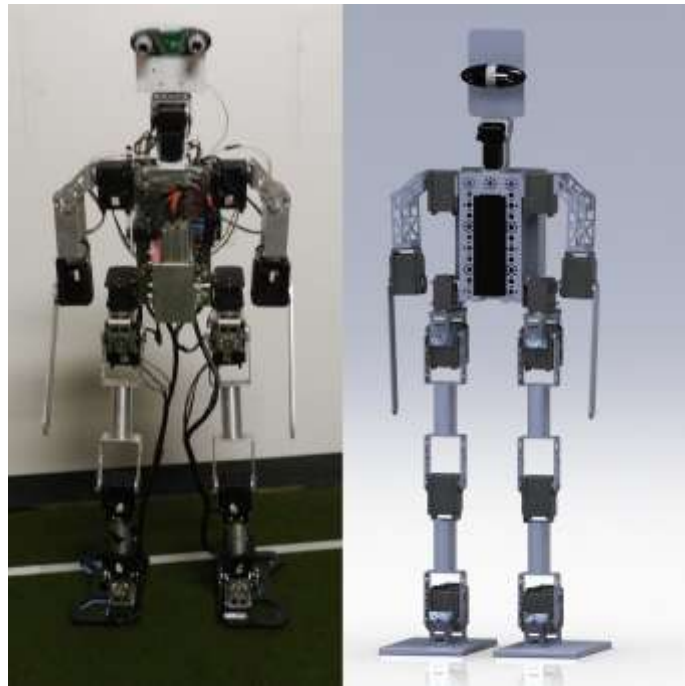
Fig. 1 a) Robot design; b) Fully built robot.
