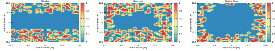
Fig. 4. Stability maps of the sampled impulse space. The red regions mark pushes that brought the robot to fall in a standing experiment (left), an open-loop walk experiment (center), and a closed-loop experiment (right).
