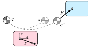
Fig. 3. The balance controller computes a zero-moment-point offset z that steers the center of mass c towards a desired state s . The next footstep location F is computed with respect to the predicted achievable end-of-step state c' .
