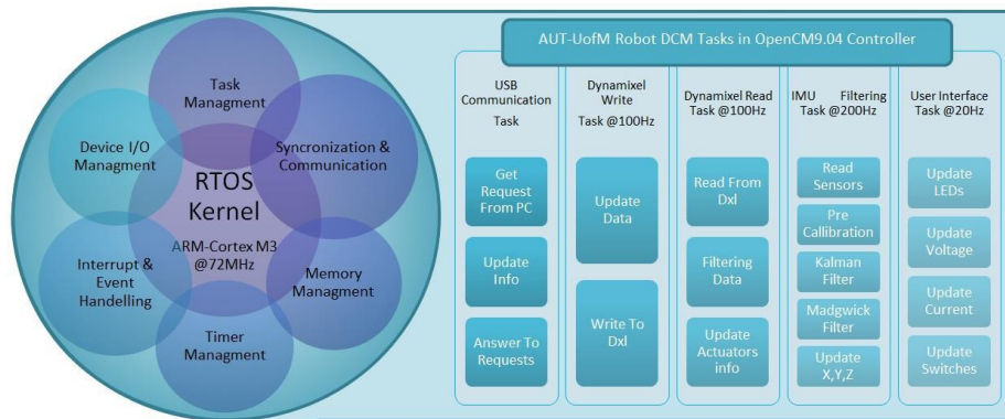
Fig. 3 OpenCM9.04 Controller internal tasks based on RTOS and filtering process diagram
