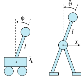
Fig. 3. The Pole-Cart model resembles the angular dynamics of the trunk during walking.
