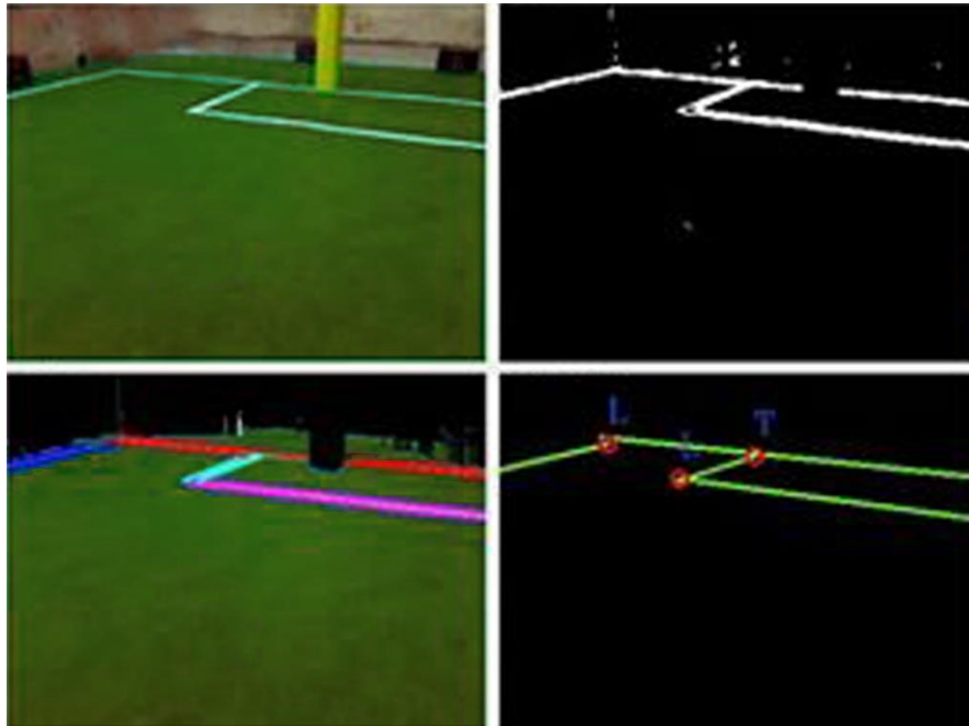
Figure 4. field features detection
