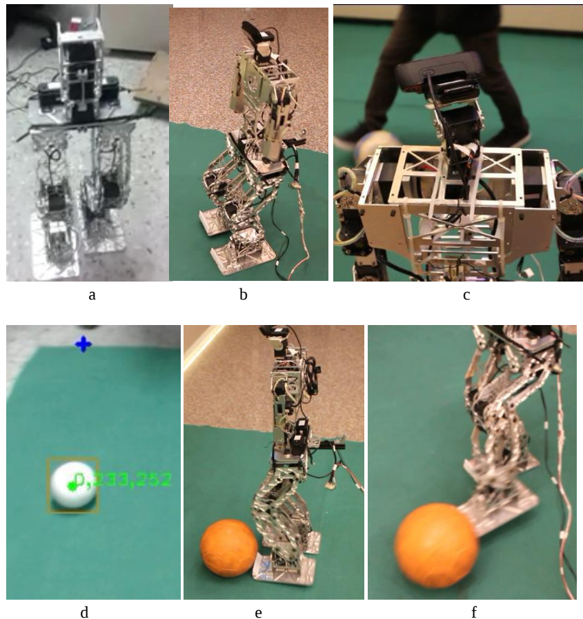
Fig. 4. Training Process: (a) Walking Training without Body. (b) Walking Training with Complete Body. (c) Tracking Ball Training. (d) White Ball Detection. (e) Dribbling Training. (f) Kicking Training
