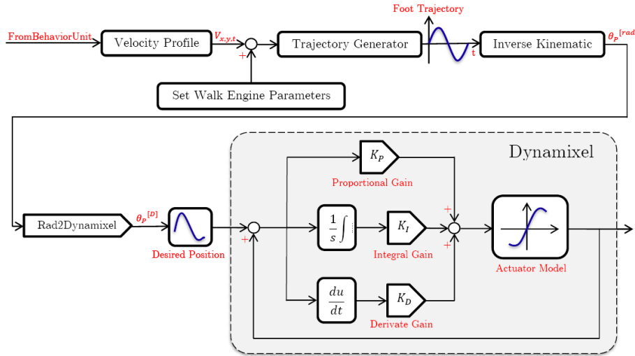
Figure 3. Walk Engine block diagram
