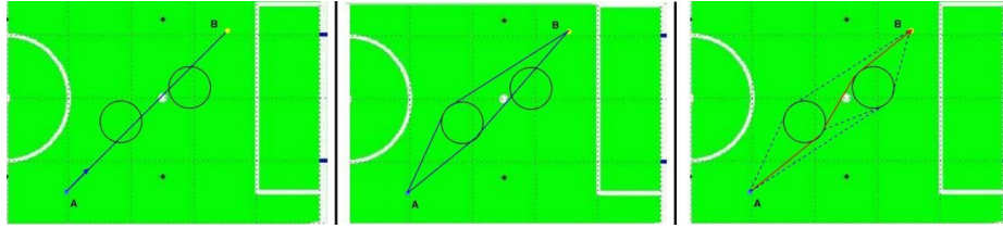
Fig. 7. Start point A and End Point B hindered by two obstacles. Drawing tangents to the first obstacle encountered o at o1 o2 o3 and o4. Recursively following the same function. Using Dijkstras Algorithm to find the final path in Red.
