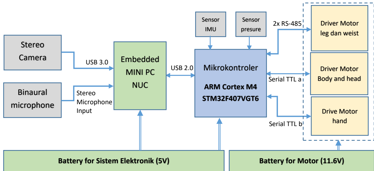
Figure 4. Overall system configuration of T-FloW
