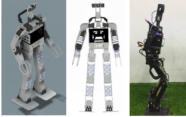
Fig. 2. Left and Centre: CAD Design of Ichiro TeenSize. Right: Ichiro TeenSize.
