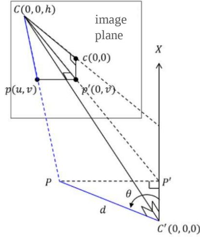
Fig. 4. Geometric method
