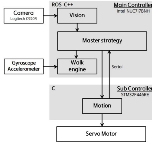
Fig. 1. overall system of robot
