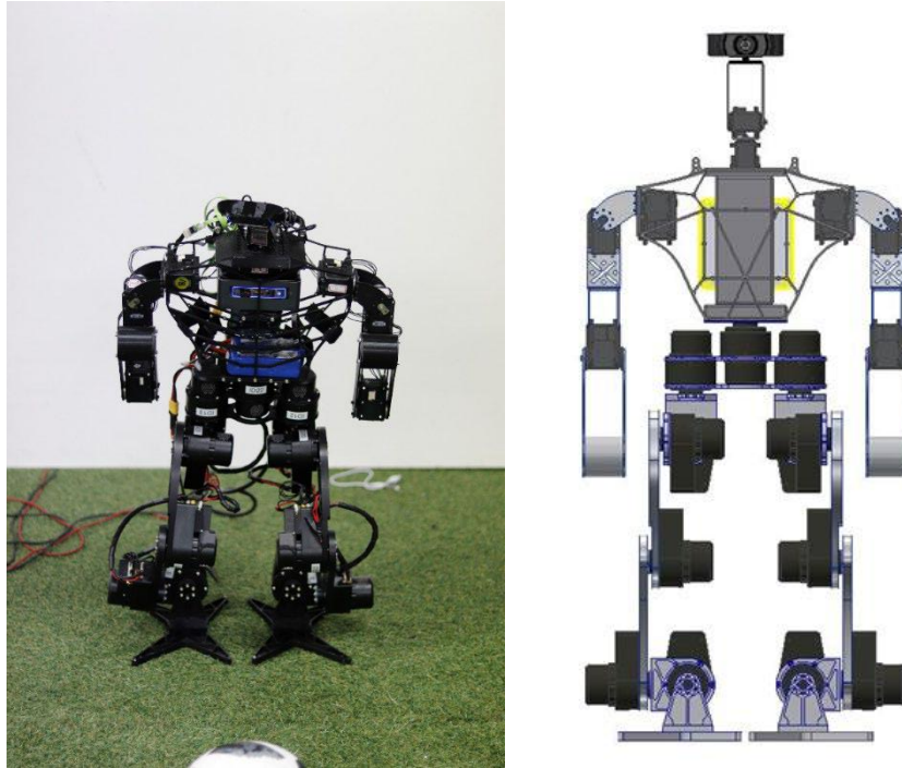
Fig. 2. Left: real picture of robot Right: design of robot
