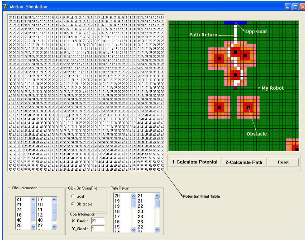
Fig.4. Trajectory Algorithm
