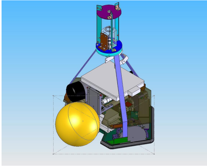
Figure 2. New Hardware Platform for the Brainstormers Tribots team
