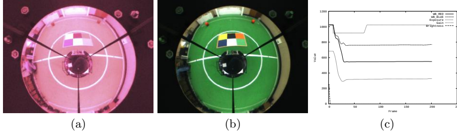
Fig. 5. An example of the autonomous configuration algorithm obtained starting with all the parameters of the camera set to the maximum value. In (a) the initial image acquired. In (b) the image obtained after applying the autonomous calibration procedure. In (c) a graphics representing the evolution of the parameters along the time.
