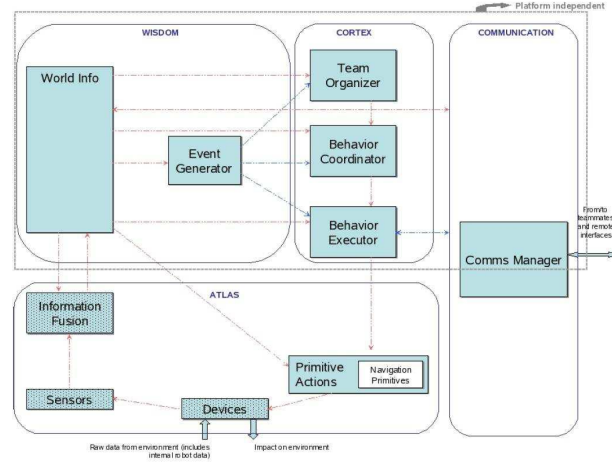
Fig. 1. Block diagram of the MeRMaID functional architecture. The block denotes main modules, denotes active objects, denotes multiple active objects, and denotes general objects (in object-oriented programming conventions). The → indicates data flow, while → indicates events flow.
